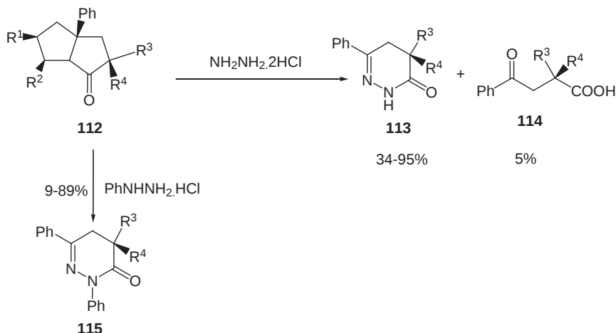
Scheme 20
