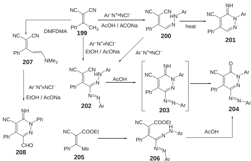
Scheme 37
