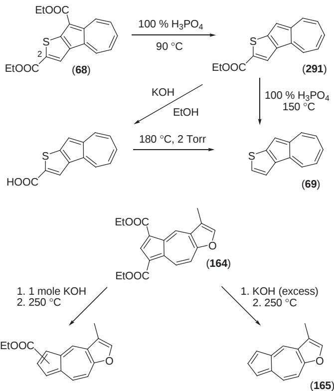
Scheme 72
