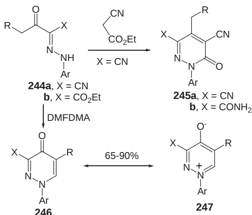
Scheme 44
