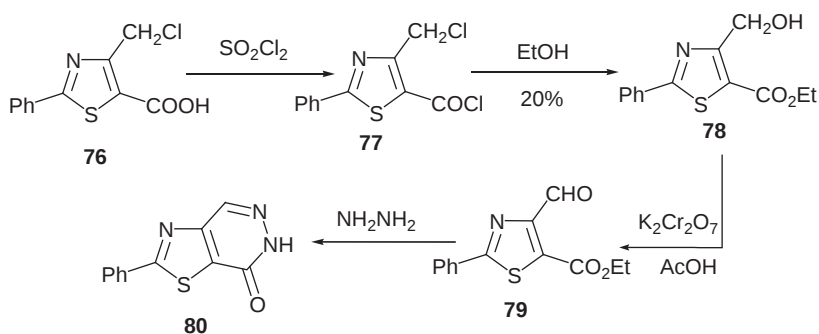
Scheme 14
