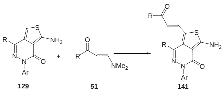
Scheme 25
