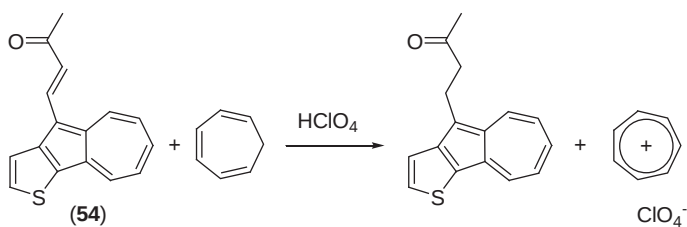
Scheme 81
