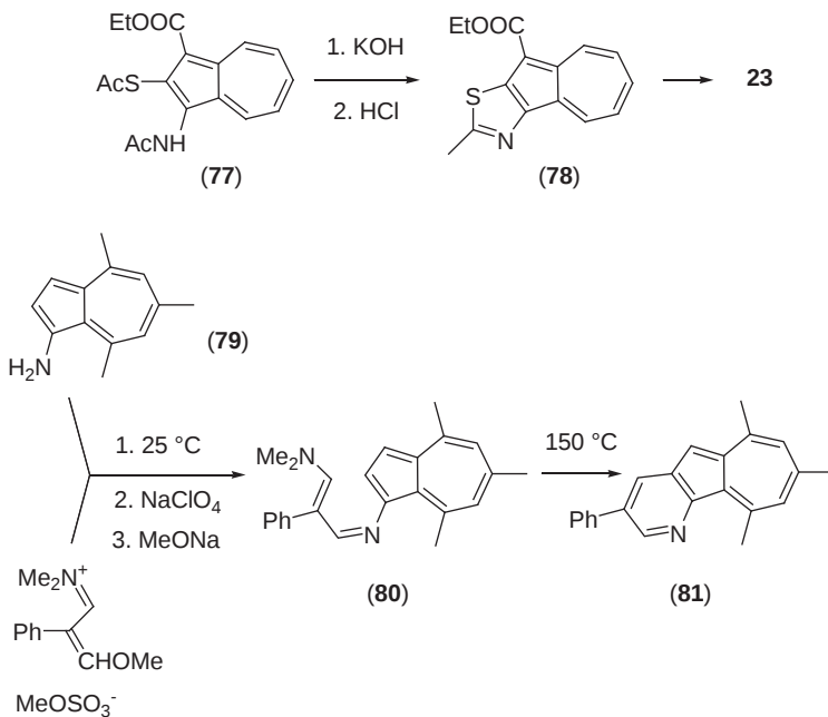
Scheme 20
