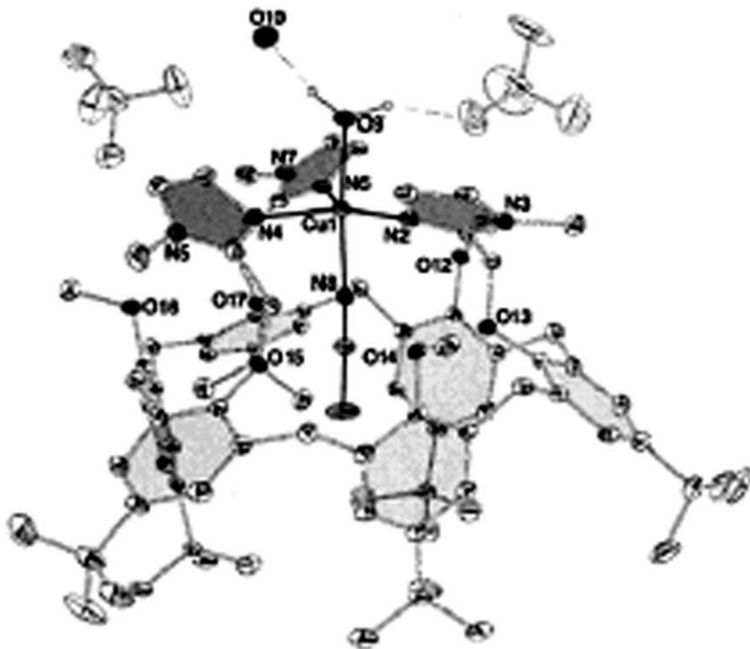
Figure 4 X-ray crystal structure of 92 . [2000IC3436] Reproduced by permission from American Chemical Society.
