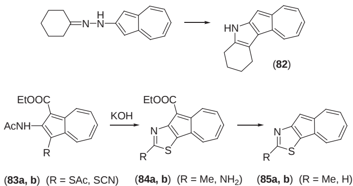
Scheme 21
