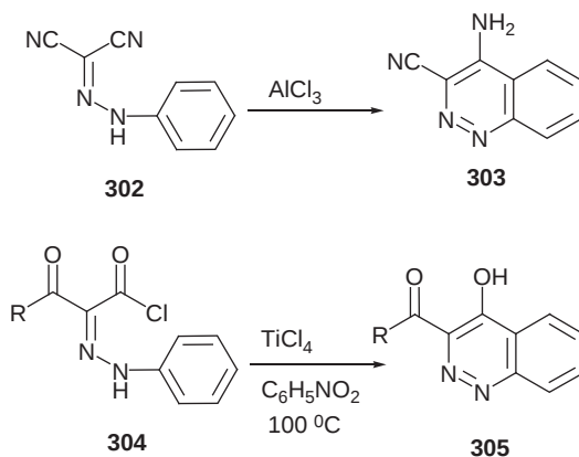
Scheme 54
