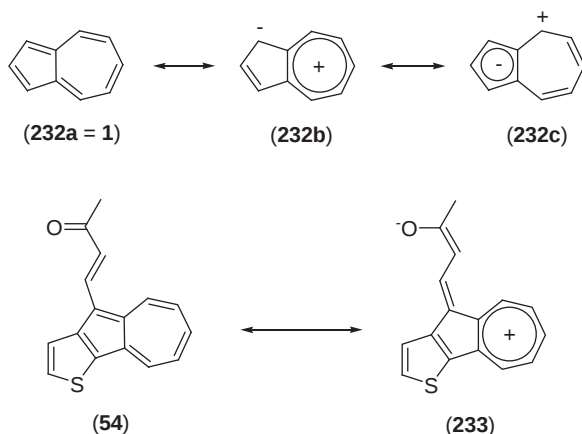
Scheme 56
