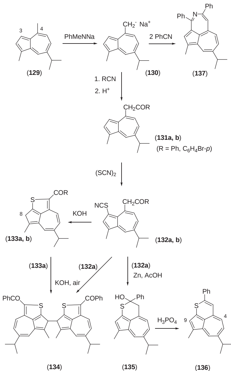
Scheme 32
