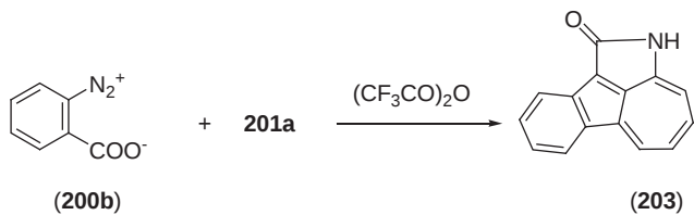
Scheme 46
