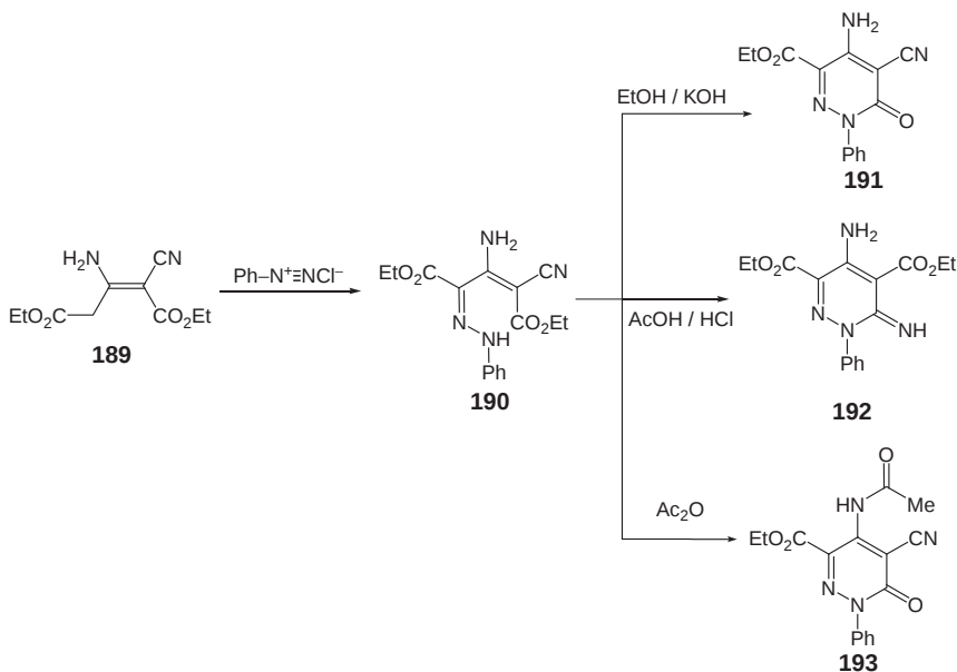
Scheme 35
