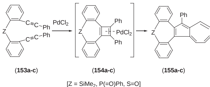
Scheme 35
