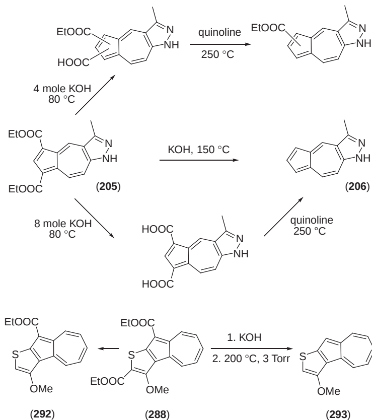
Scheme 73
