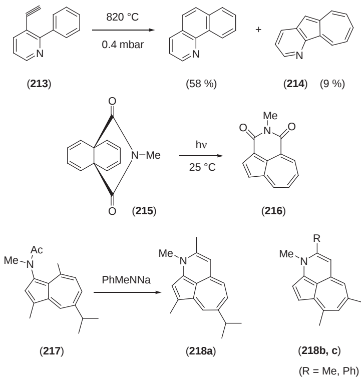
Scheme 49
