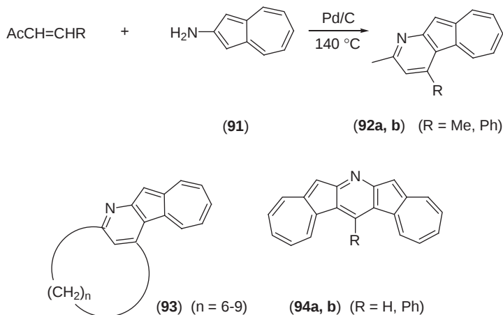
Scheme 23
