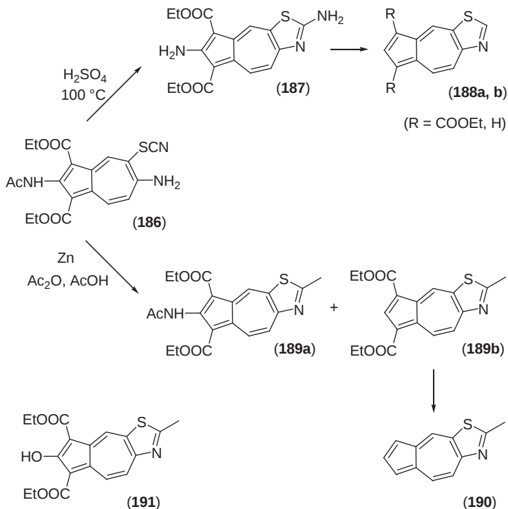
Scheme 43
