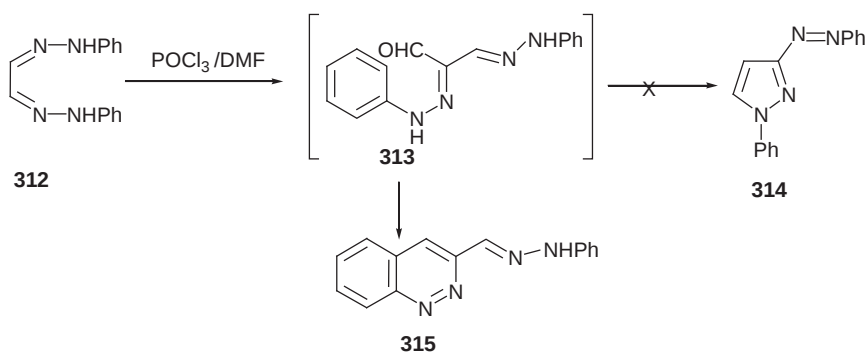
Scheme 56
