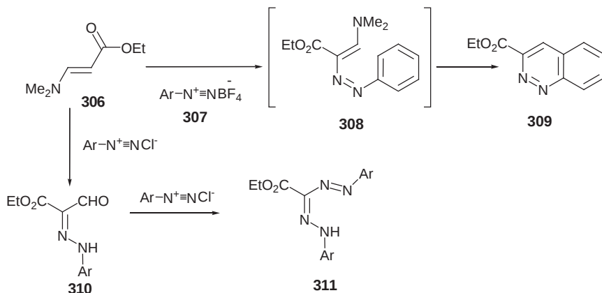
Scheme 55
