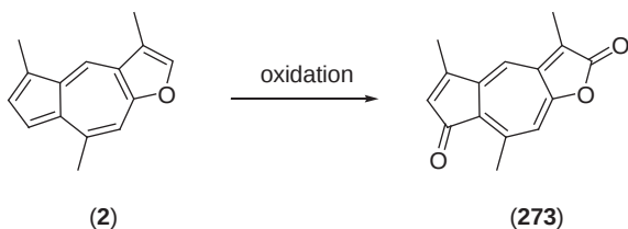
Scheme 67
