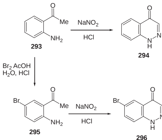
Scheme 53
