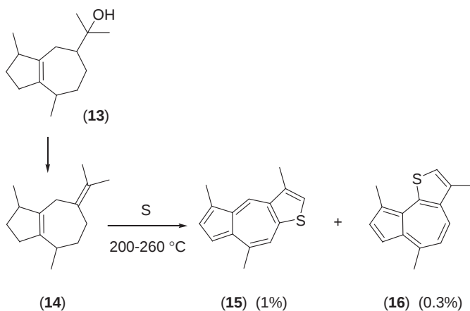
Scheme 6
