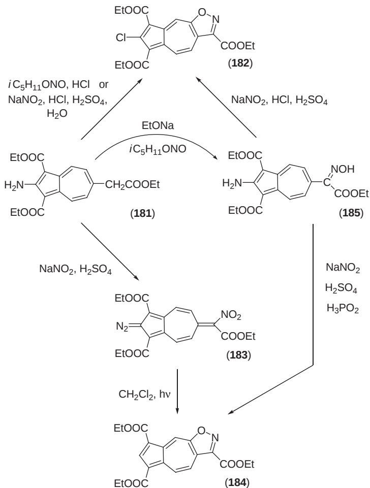
Scheme 42
