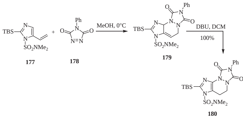
Scheme 32
