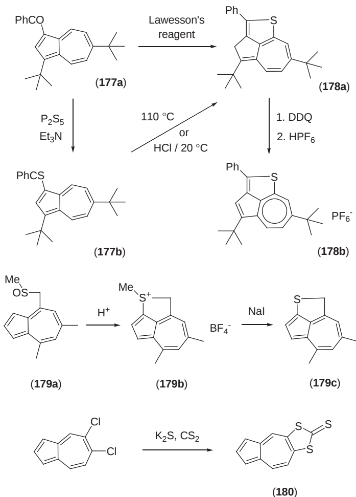
Scheme 41
