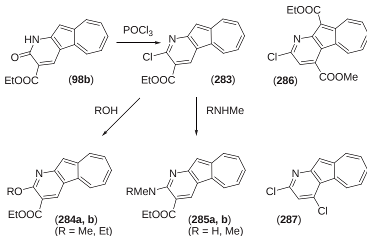
Scheme 70
