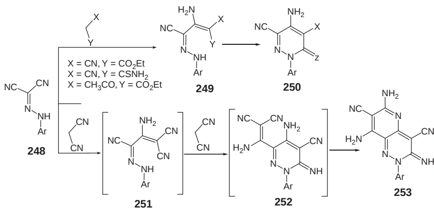
Scheme 45
