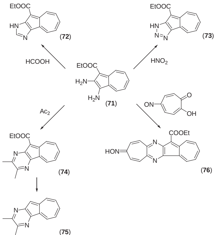
Scheme 19
