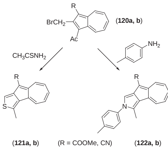
Scheme 29
